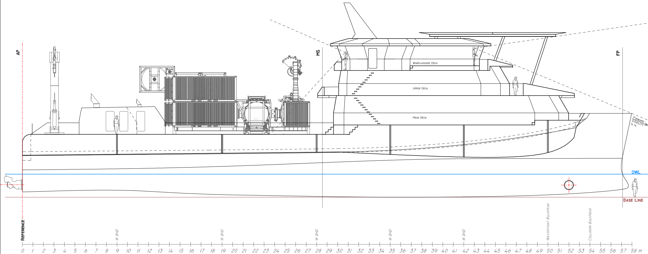
SHIP AXIS SECTION
